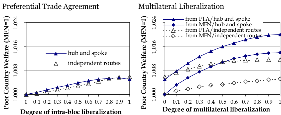
Figures A.3. “hub-and-spoke” vs. “independent routes” transport network. ( t=0.3 , k=3 , \alpha=0.5 , \theta=0.75 , C=4 , N_r=N_p=16 , B=4 )
